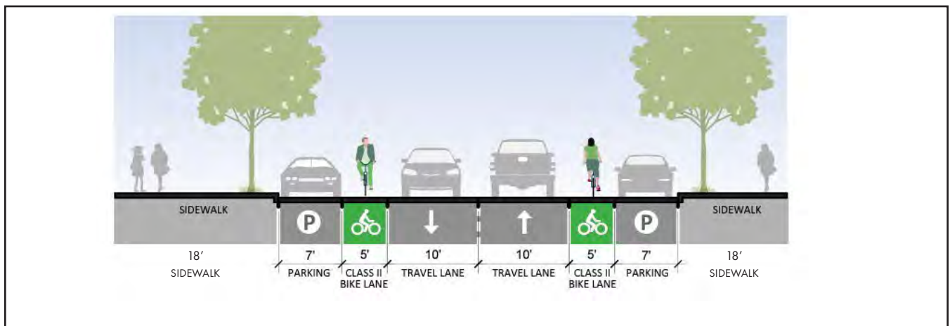
Figure 7.6: Pioneer Blvd. Cross-Section from SGL ROW to 500' south of 183rd St., Illustrative Class II Bike Lanes Street Source: SGL FLM Plan, released 2024, page 251.
