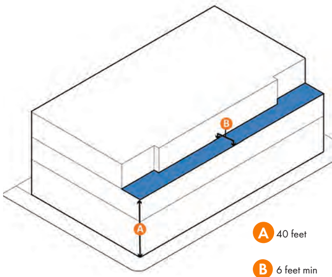
Figure 6.10: Stepback
