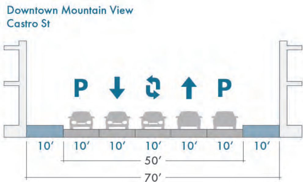
Figure 2.15: Castro Street Existing Street Section
