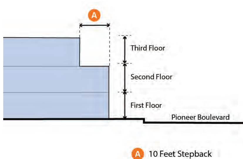
Figure 6.4: Special Setback A for properties fronting Pioneer Boulevard
