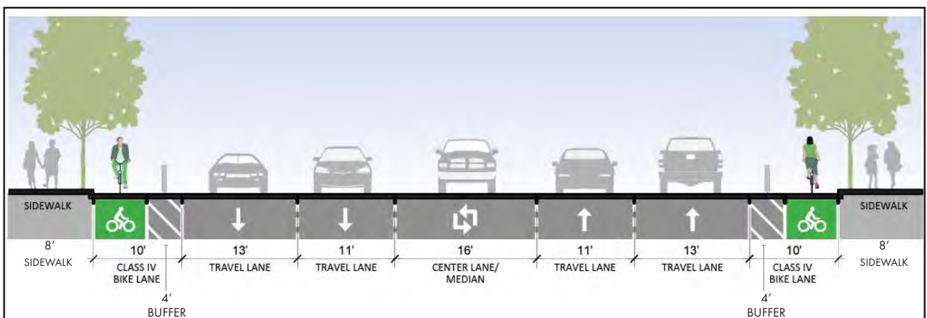
Figure 7.7: Pioneer Blvd. Cross-Section from South St. to Del Amo Blvd., Illustrative Class IV Bike Lanes Source: SGL FLM Plan, released 2024, page 252.
