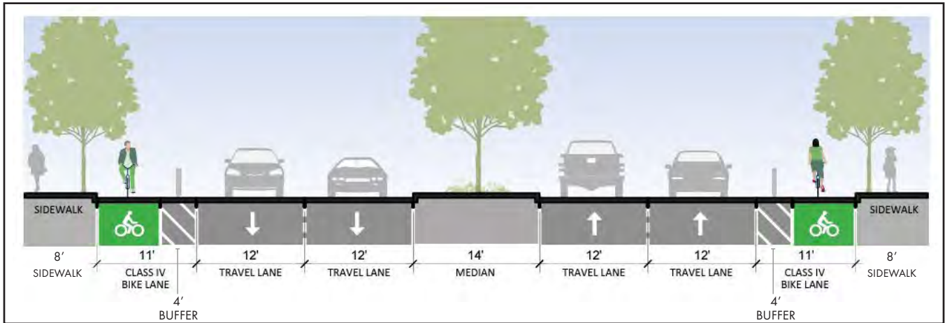
Figure 7.5: Pioneer Blvd. Cross Section from 166th St to 500' south of 183rd St., Illustrative Class IV Bike Lanes Source: SGL FLM Plan, released 2024, page 250.
