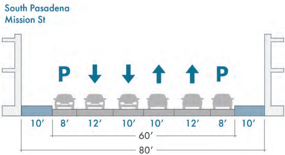
Figure 2.12: Mission Street Existing Street Section
